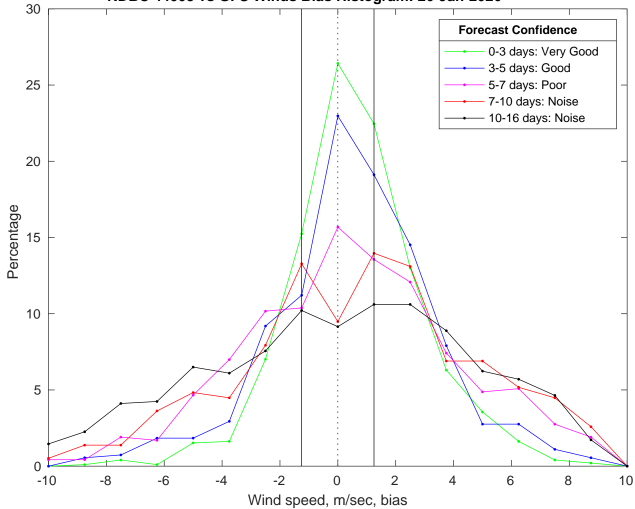
NDBC 44008 vs GFS Winds Bias Histogram: 26-Jan-2026
