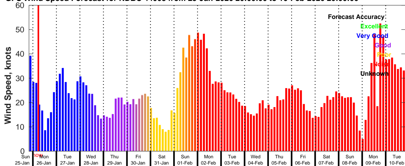
GFS Wind Speed Forecast for NDBC 44008 from 25-Jan-2026 20:00:00 to 10-Feb-2026 20:00:00
