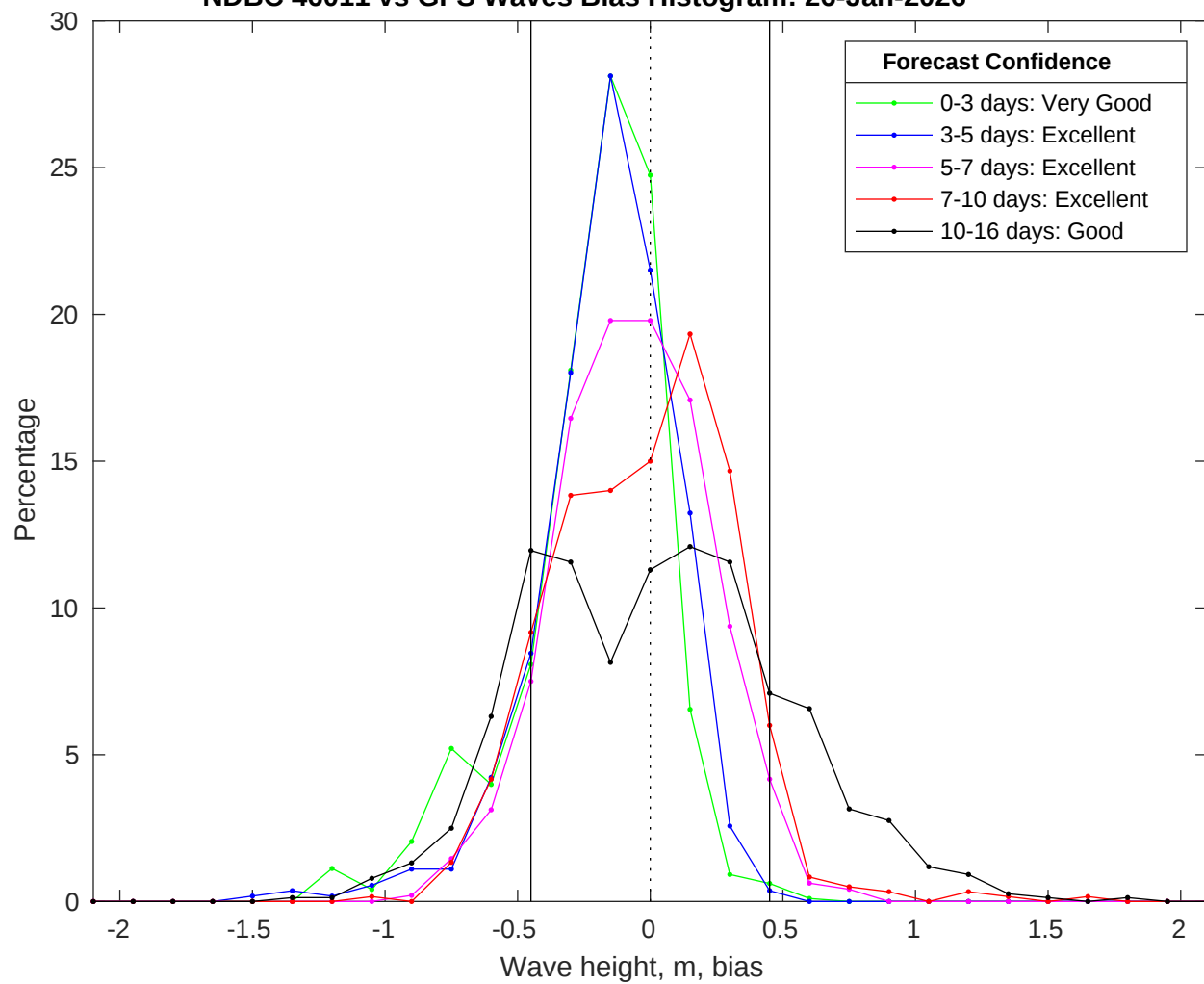
NDBC 46011 vs GFS Waves Bias Histogram: 26-Jan-2026
