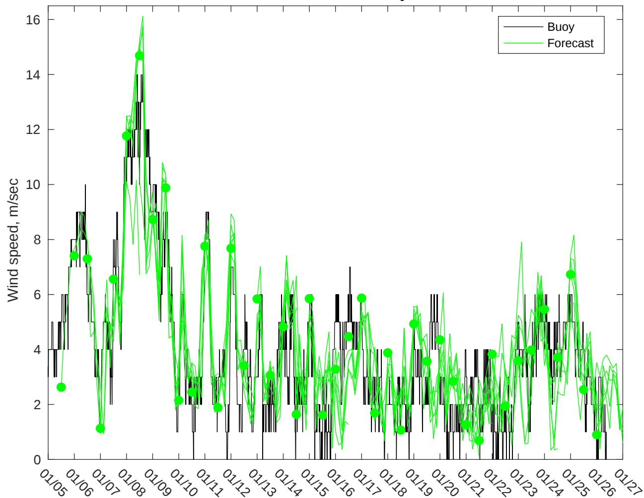
NDBC 46011 vs GFS Winds: 0 to 3 day forecast
