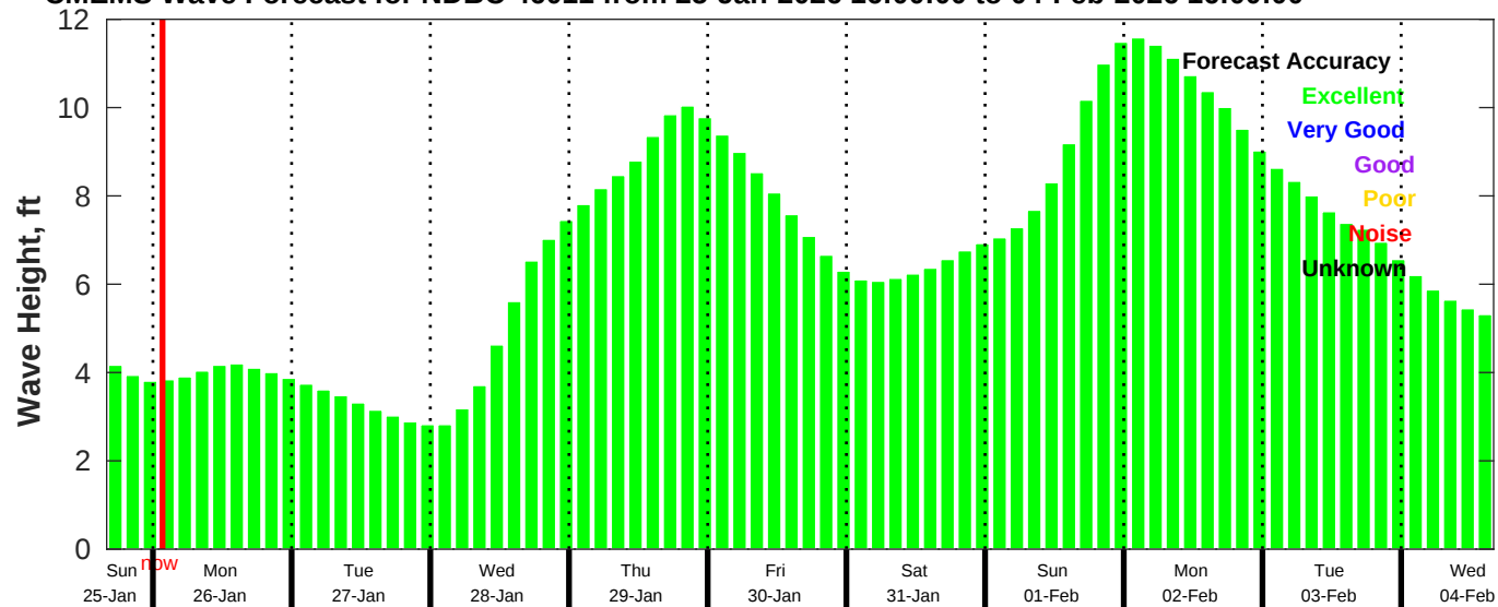
CMEMS Wave Forecast for NDBC 46011 from 25-Jan-2026 16:00:00 to 04-Feb-2026 16:00:00
