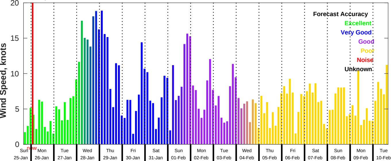
GFS Wind Speed Forecast for NDBC 46011 from 25-Jan-2026 16:00:00 to 10-Feb-2026 16:00:00
