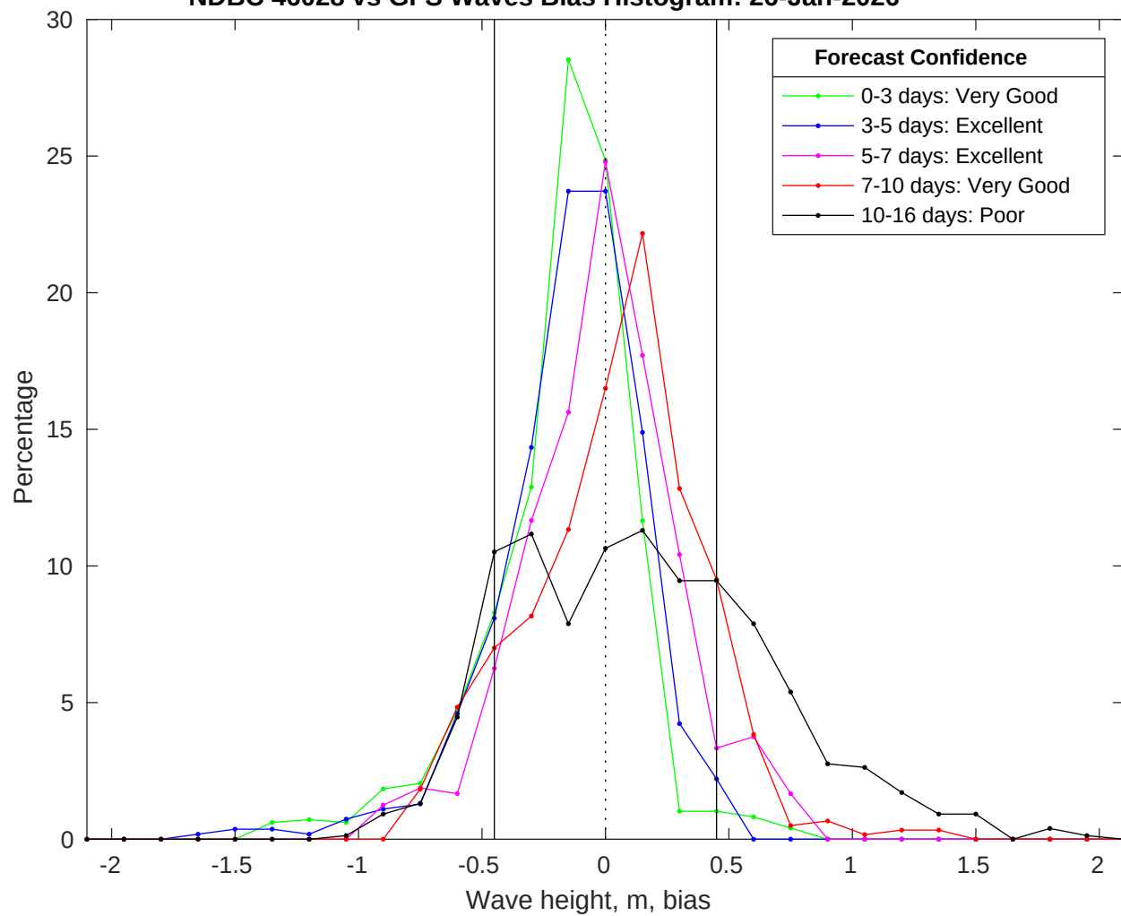
NDBC 46028 vs GFS Waves Bias Histogram: 26-Jan-2026
