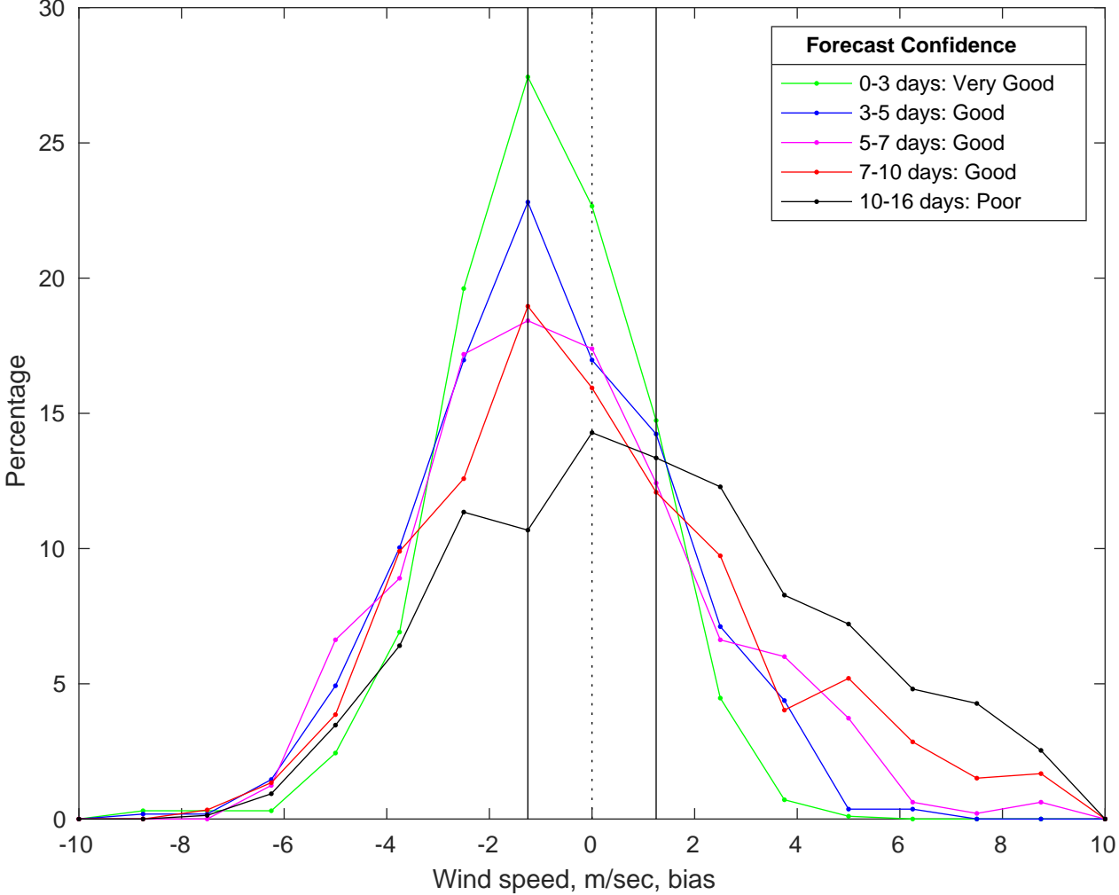
NDBC 46028 vs GFS Winds Bias Histogram: 26-Jan-2026
