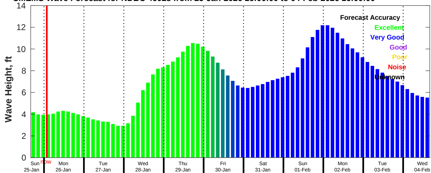
CMEMS Wave Forecast for NDBC 46028 from 25-Jan-2026 16:00:00 to 04-Feb-2026 16:00:00
