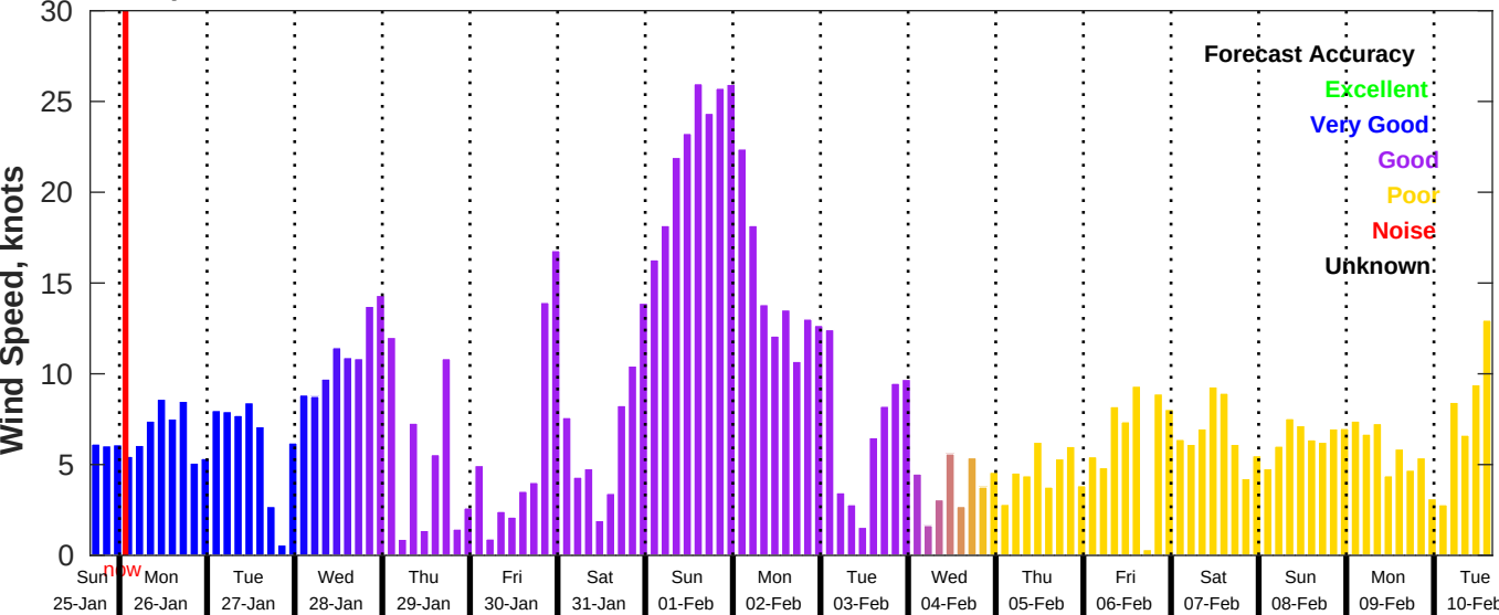
GFS Wind Speed Forecast for NDBC 46028 from 25-Jan-2026 16:00:00 to 10-Feb-2026 16:00:00
