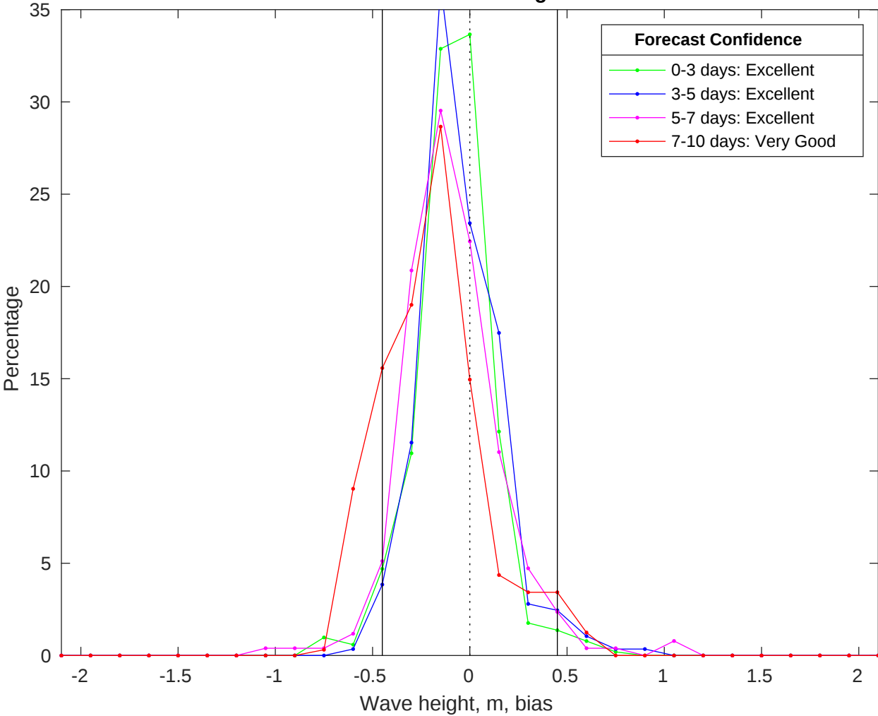
NDBC 46054 vs CMEMS Waves Bias Histogram: 26-Jan-2026
