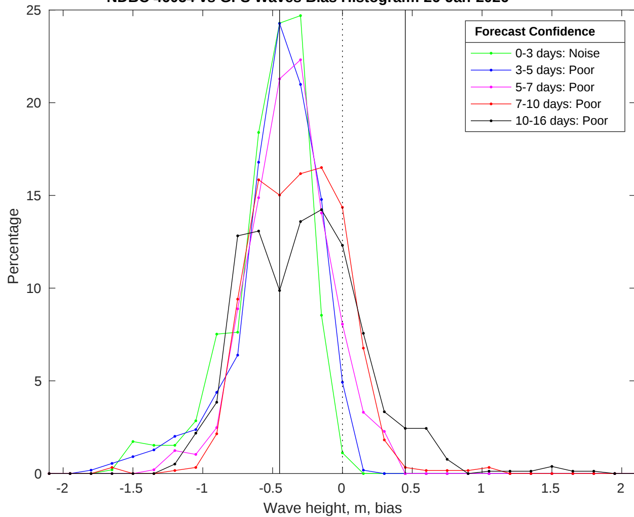
NDBC 46054 vs GFS Waves Bias Histogram: 26-Jan-2026
