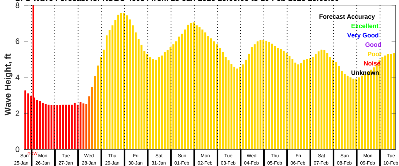
GFS Wave Forecast for NDBC 46054 from 25-Jan-2026 16:00:00 to 10-Feb-2026 16:00:00
