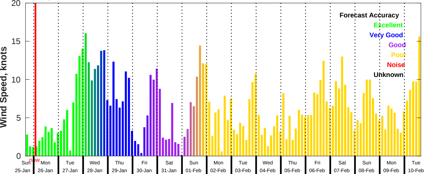
GFS Wind Speed Forecast for NDBC 46054 from 25-Jan-2026 16:00:00 to 10-Feb-2026 16:00:00
