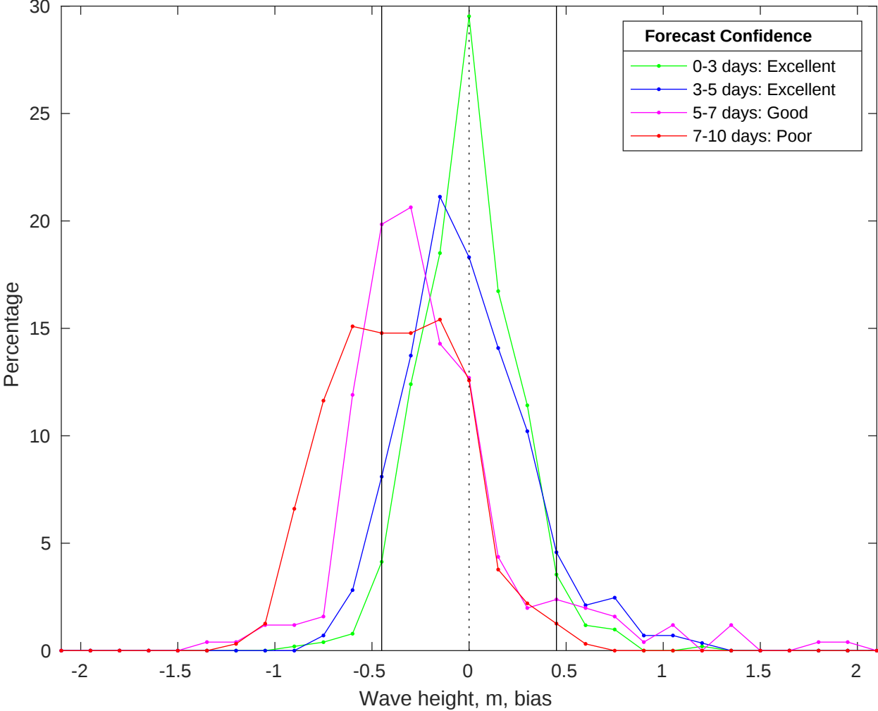
NDBC 46059 vs CMEMS Waves Bias Histogram: 26-Jan-2026
