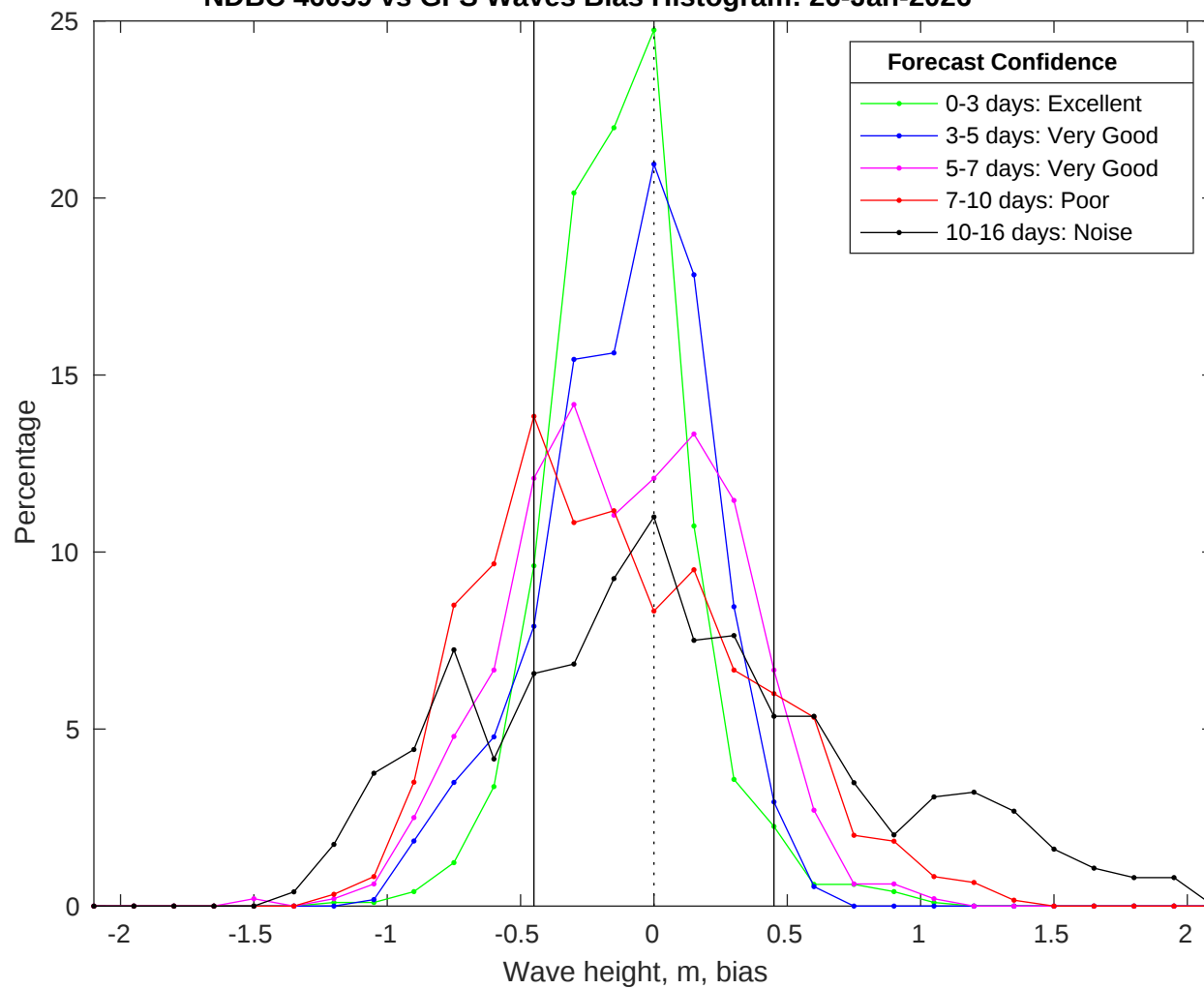
NDBC 46059 vs GFS Waves Bias Histogram: 26-Jan-2026
