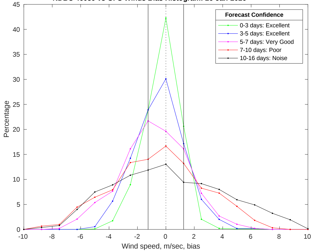
NDBC 46059 vs GFS Winds Bias Histogram: 26-Jan-2026
