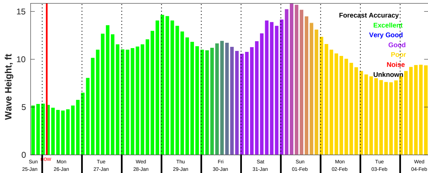
CMEMS Wave Forecast for NDBC 46059 from 25-Jan-2026 17:00:00 to 04-Feb-2026 17:00:00
