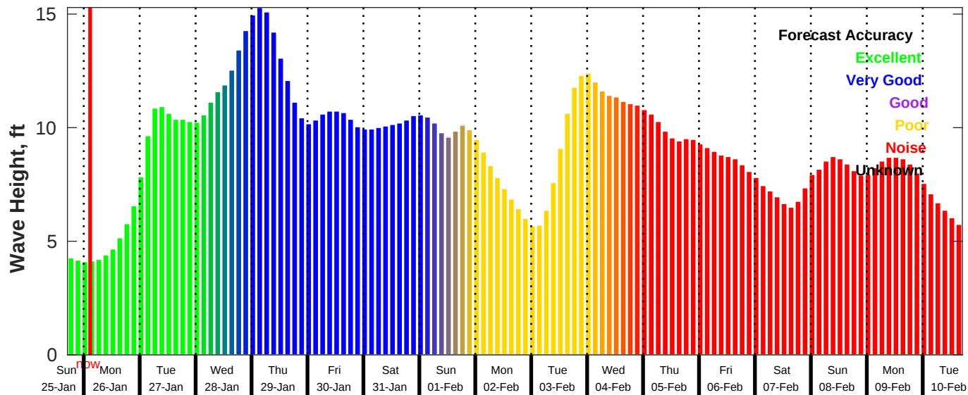
GFS Wave Forecast for NDBC 46059 from 25-Jan-2026 17:00:00 to 10-Feb-2026 17:00:00
