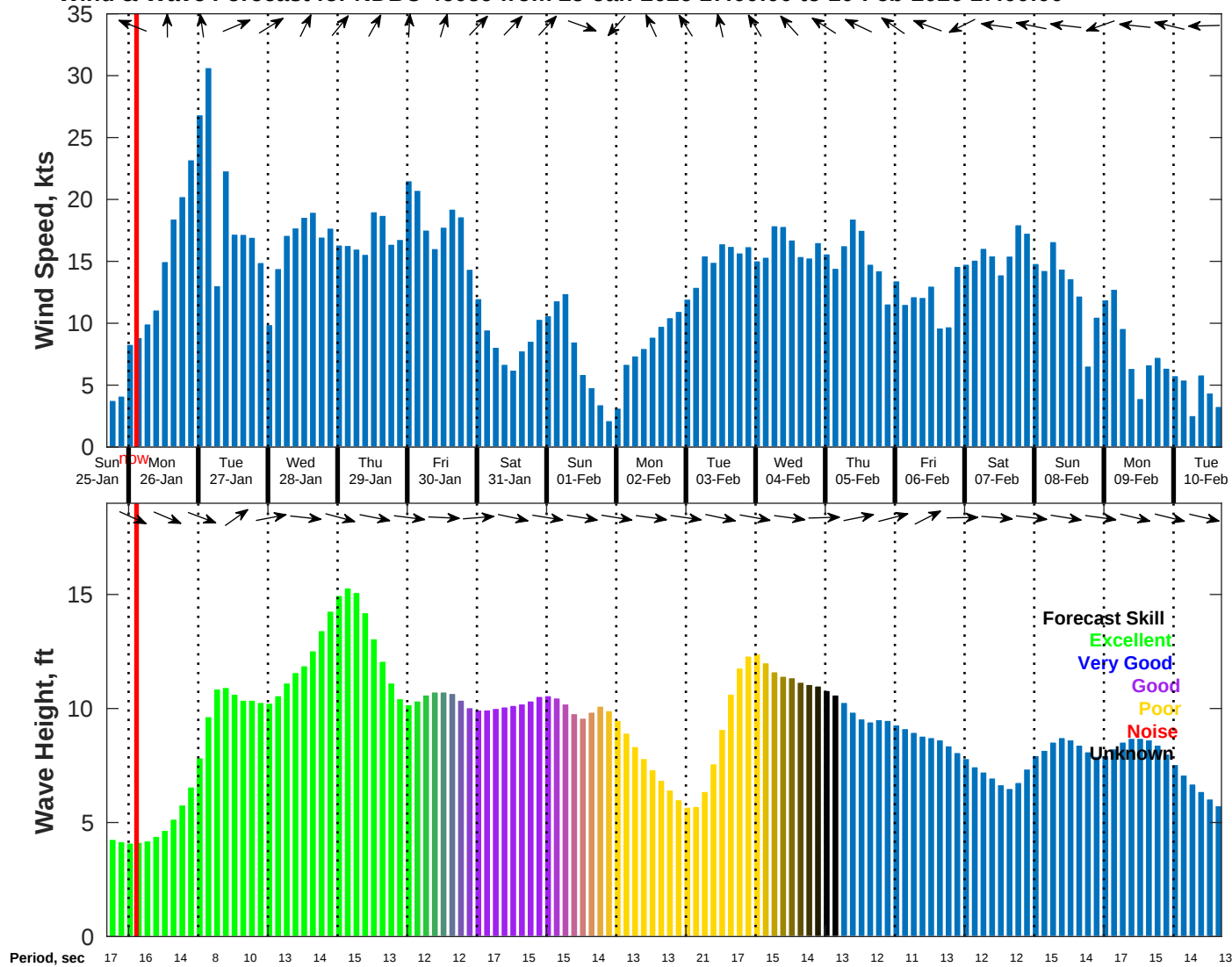
Wind & Wave Forecast for NDBC 46059 from 25-Jan-2026 17:00:00 to 10-Feb-2026 17:00:00
