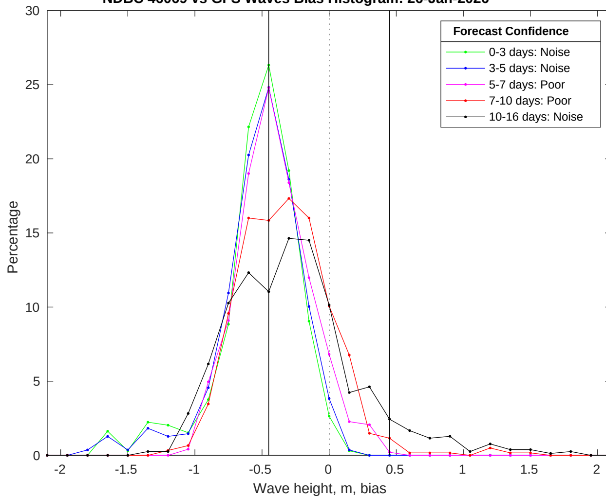
NDBC 46069 vs GFS Waves Bias Histogram: 26-Jan-2026
