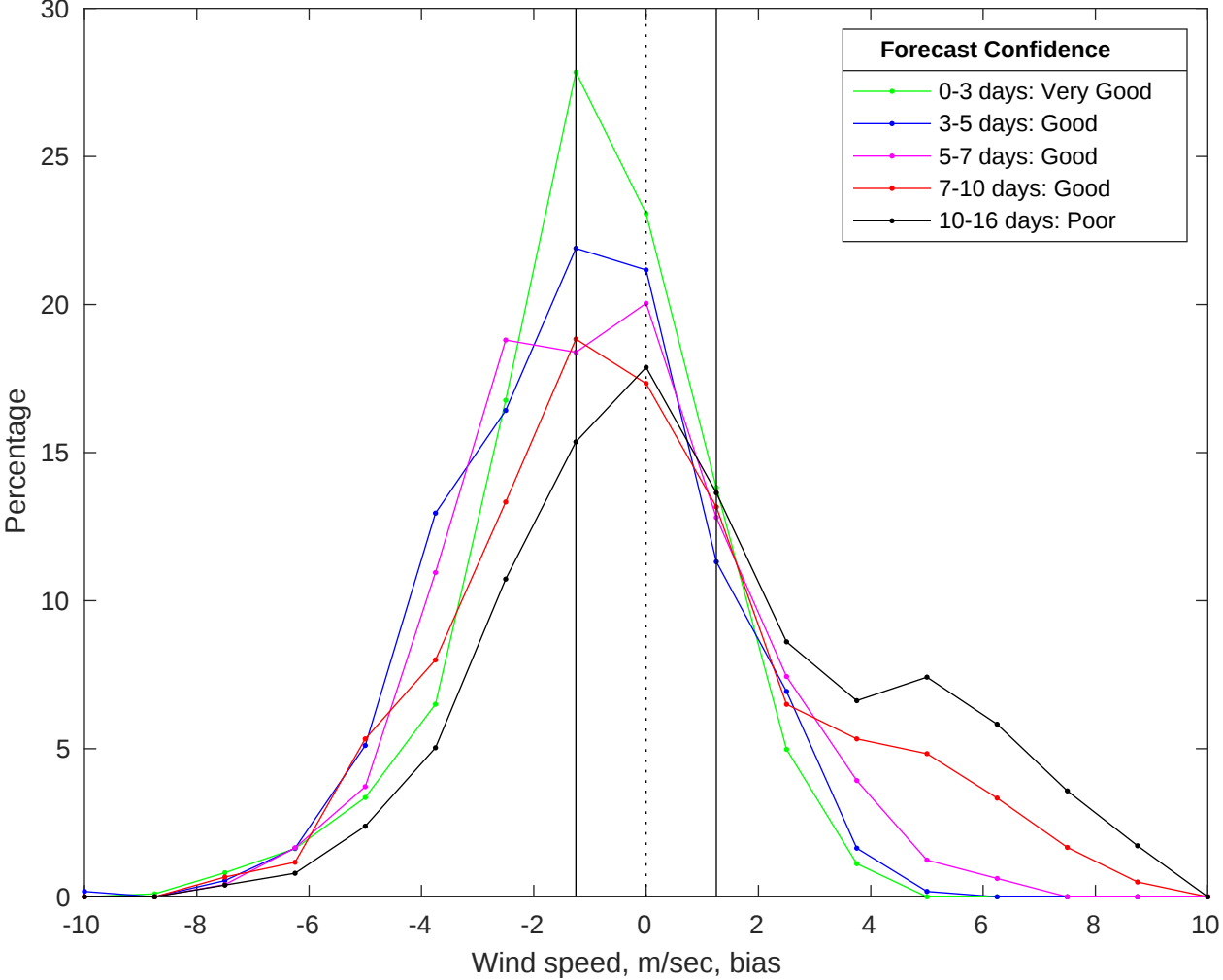
NDBC 46069 vs GFS Winds Bias Histogram: 26-Jan-2026
