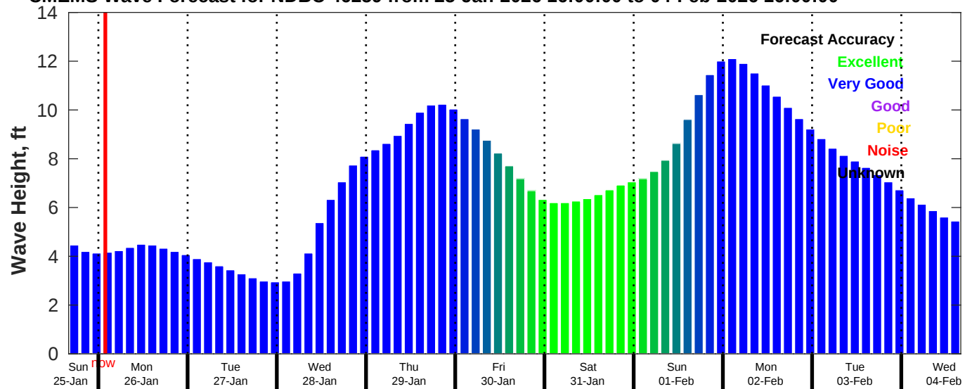
CMEMS Wave Forecast for NDBC 46259 from 25-Jan-2026 16:00:00 to 04-Feb-2026 16:00:00
