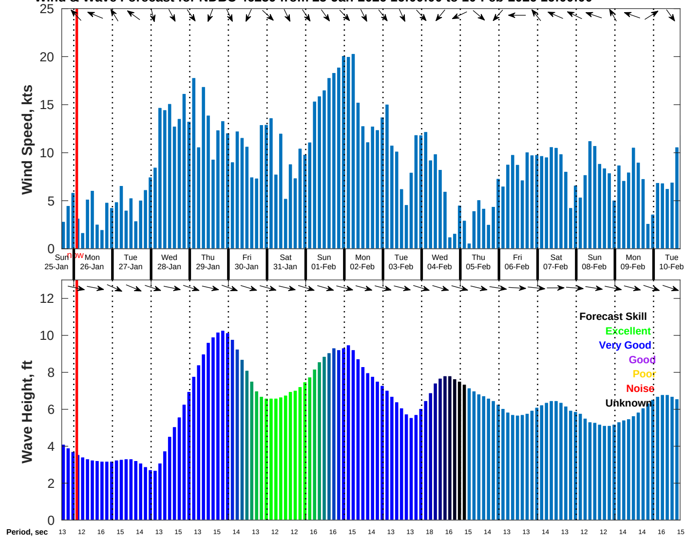
Wind & Wave Forecast for NDBC 46259 from 25-Jan-2026 16:00:00 to 10-Feb-2026 16:00:00
