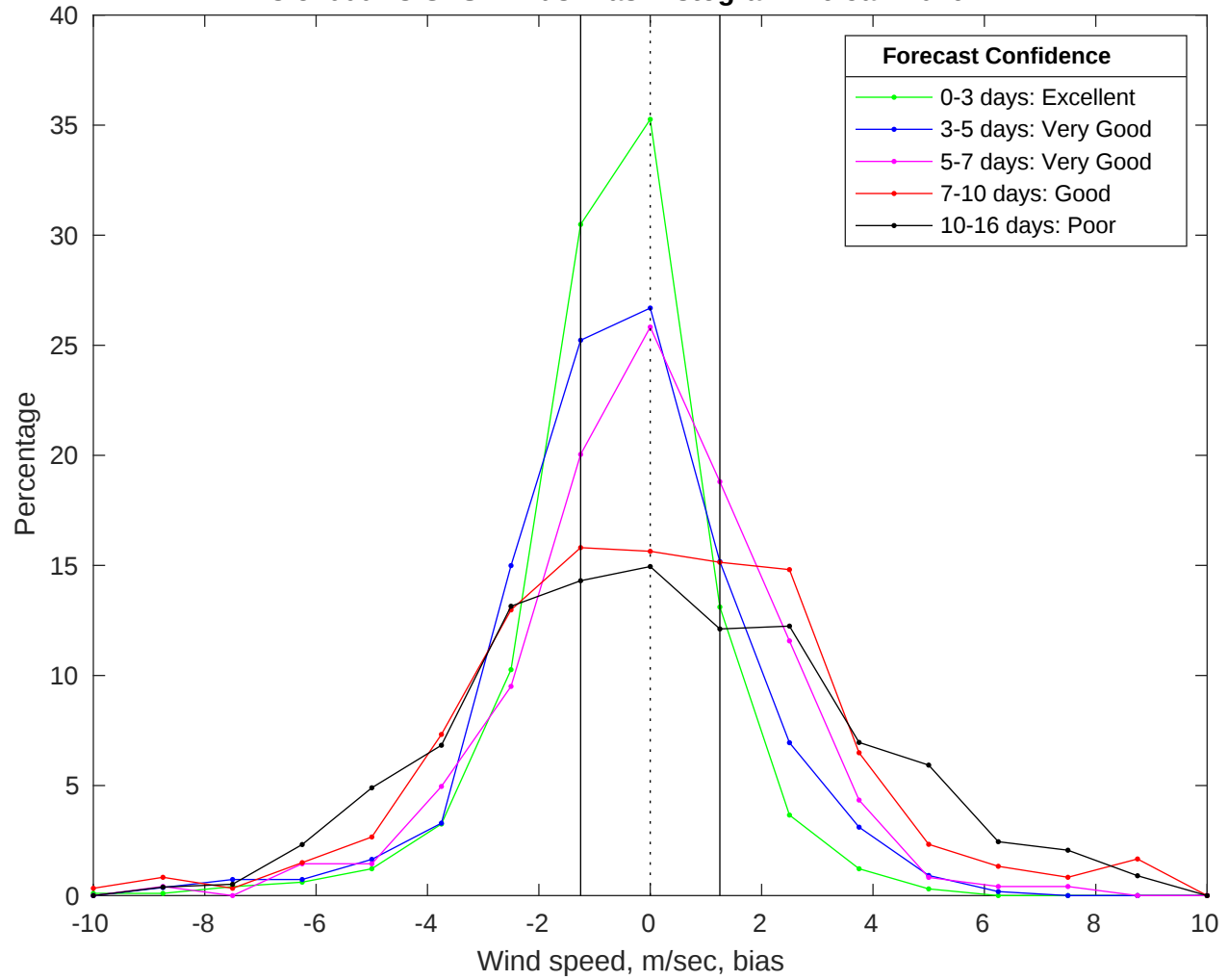
NDBC 51000 vs GFS Winds Bias Histogram: 26-Jan-2026
