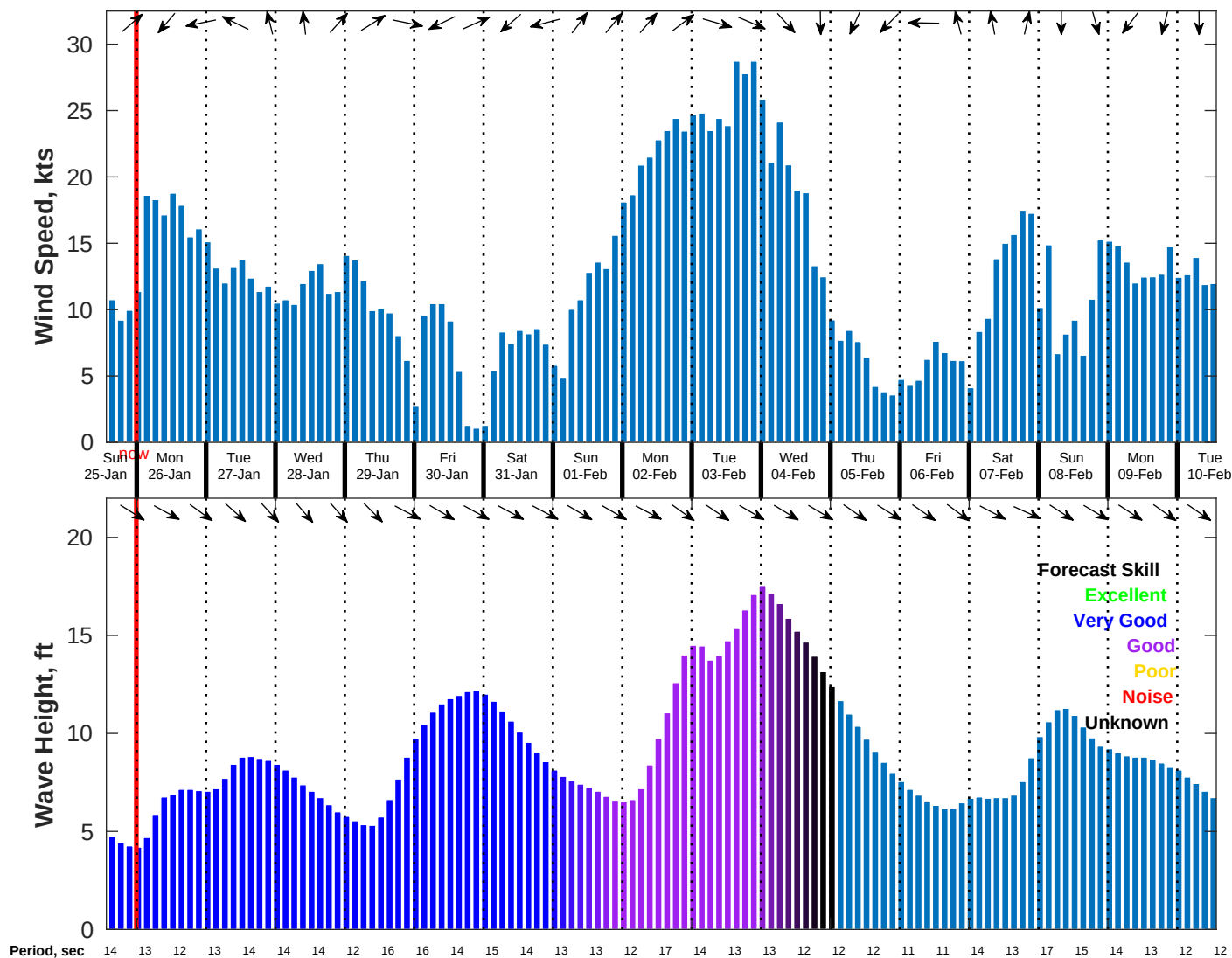
Wind & Wave Forecast for NDBC 51000 from 25-Jan-2026 14:00:00 to 10-Feb-2026 14:00:00
