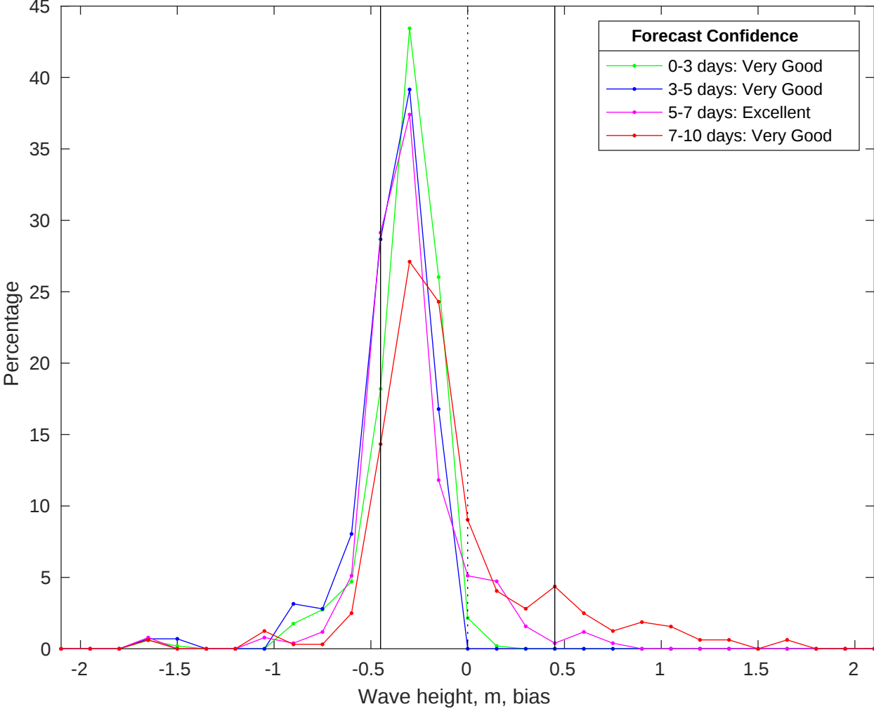
NDBC 51209 vs CMEMS Waves Bias Histogram: 26-Jan-2026
