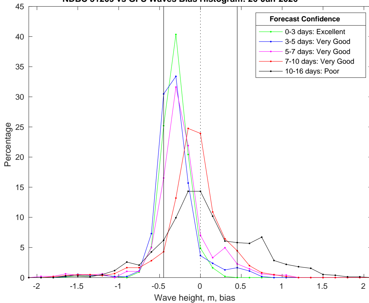
NDBC 51209 vs GFS Waves Bias Histogram: 26-Jan-2026
