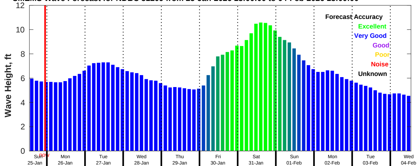
CMEMS Wave Forecast for NDBC 51209 from 25-Jan-2026 13:00:00 to 04-Feb-2026 13:00:00
