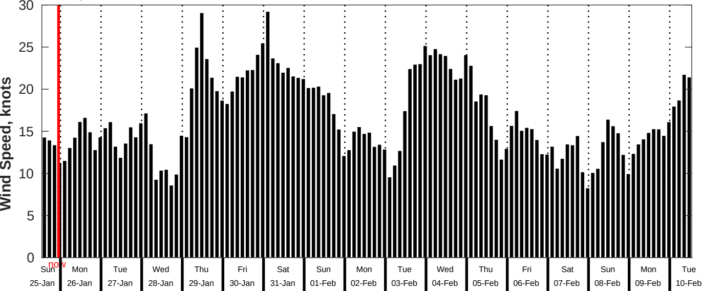
GFS Wind Speed Forecast for NDBC 51209 from 25-Jan-2026 13:00:00 to 10-Feb-2026 13:00:00
