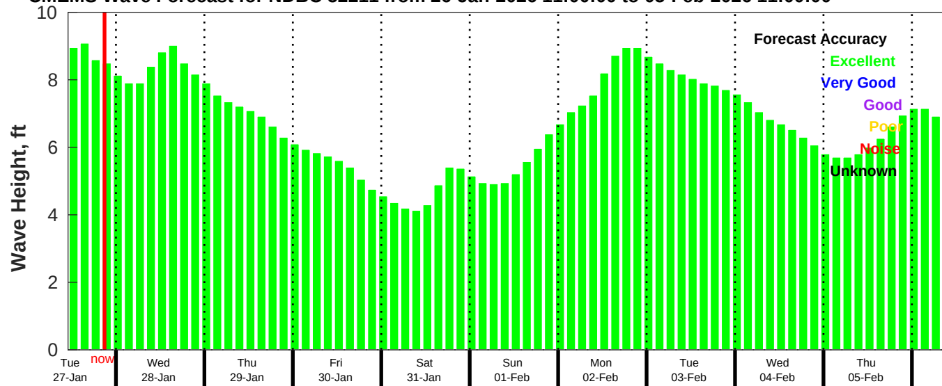
CMEMS Wave Forecast for NDBC 52211 from 26-Jan-2026 11:00:00 to 05-Feb-2026 11:00:00
