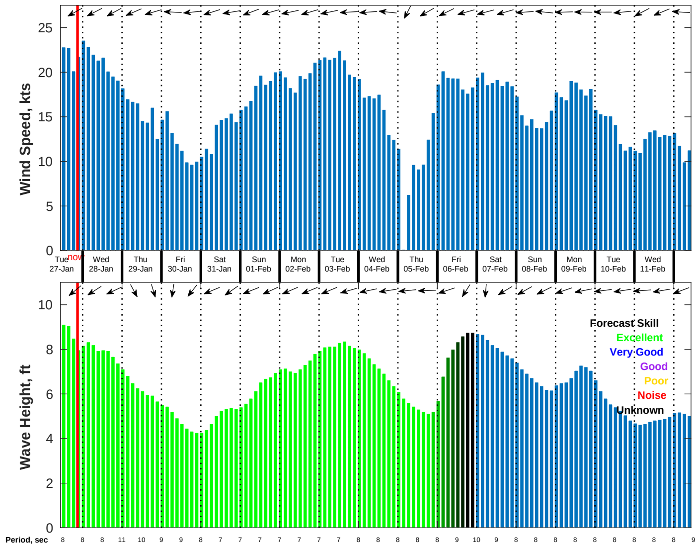
Wind & Wave Forecast for NDBC 52211 from 26-Jan-2026 11:00:00 to 11-Feb-2026 11:00:00
