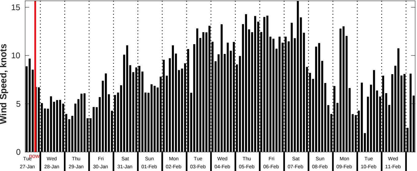
GFS Wind Speed Forecast for NDBC 52212 from 26-Jan-2026 09:00:00 to 11-Feb-2026 09:00:00
