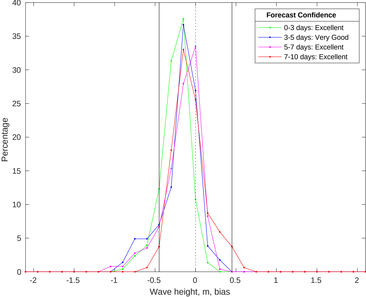
NDBC 52213 vs CMEMS Waves Bias Histogram: 26-Jan-2026
