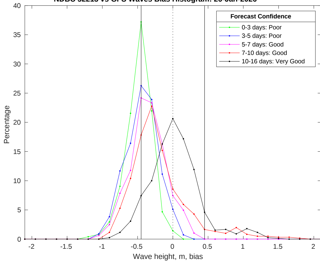
NDBC 52213 vs GFS Waves Bias Histogram: 26-Jan-2026
