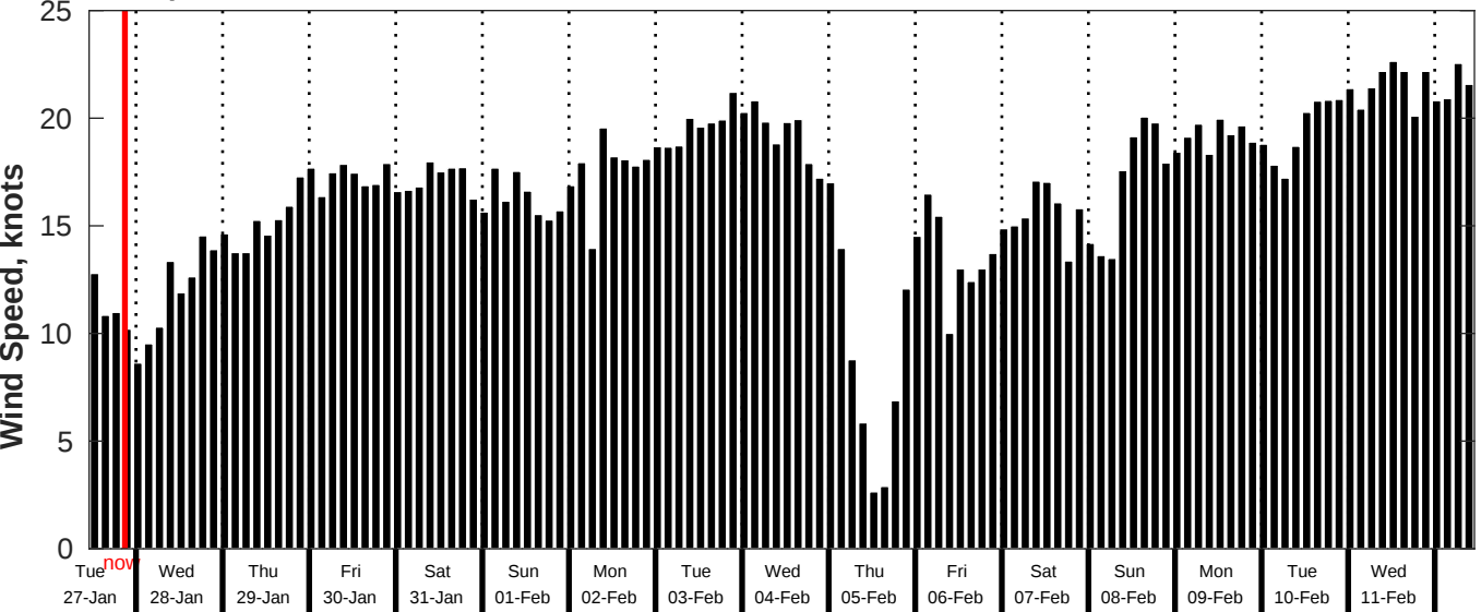
GFS Wind Speed Forecast for NDBC 52213 from 26-Jan-2026 11:00:00 to 11-Feb-2026 11:00:00
