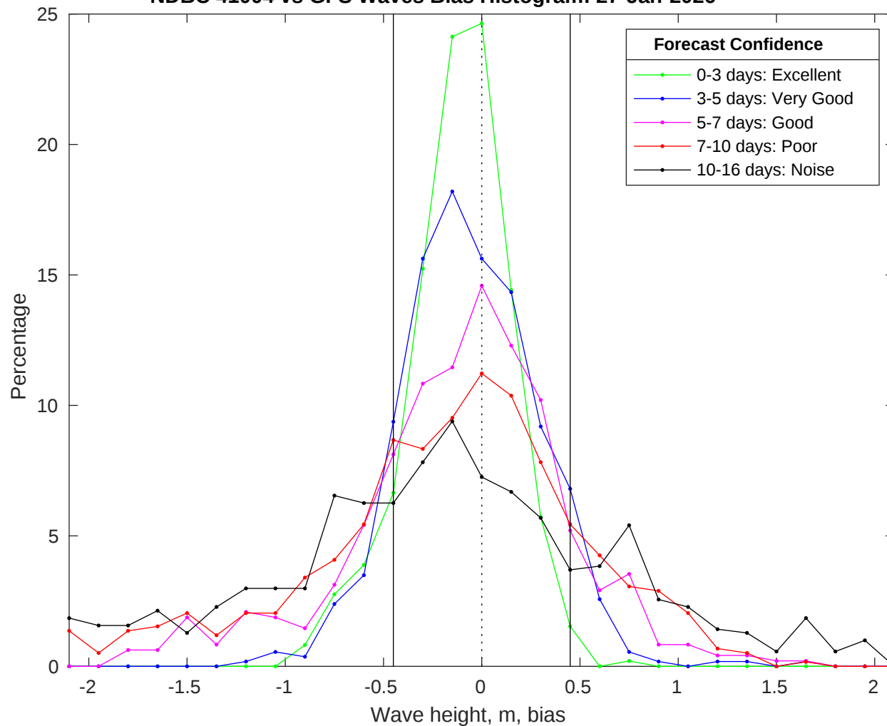
NDBC 41004 vs GFS Waves Bias Histogram: 27-Jan-2026
