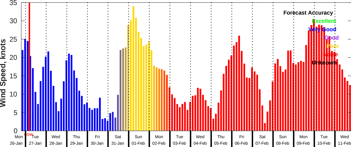
GFS Wind Speed Forecast for NDBC 41004 from 26-Jan-2026 19:00:00 to 11-Feb-2026 19:00:00
