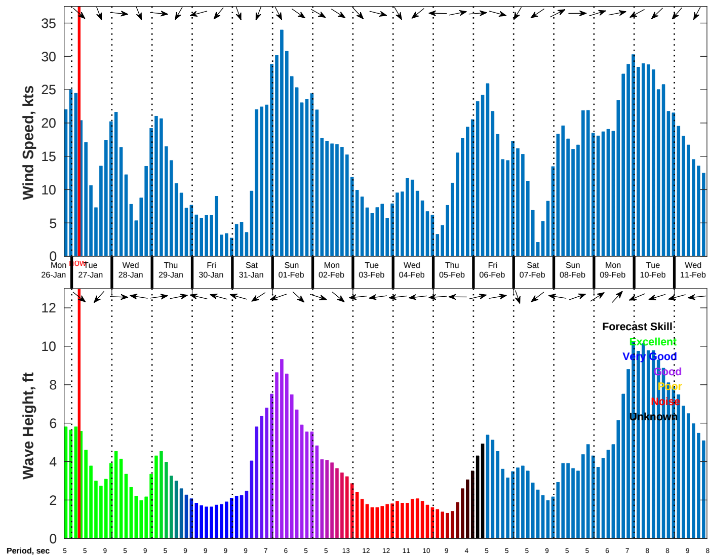
Wind & Wave Forecast for NDBC 41004 from 26-Jan-2026 19:00:00 to 11-Feb-2026 19:00:00
