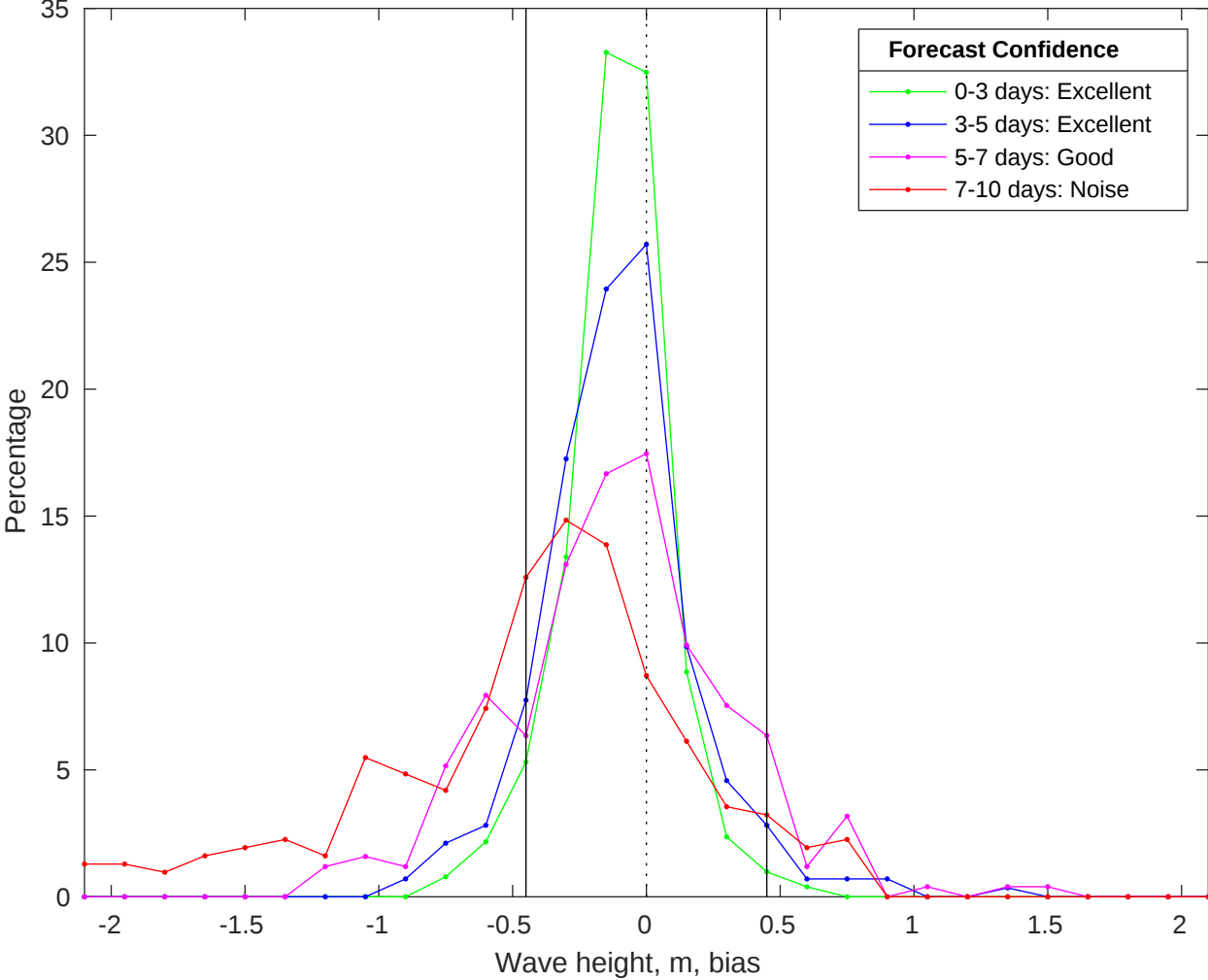
NDBC 41013 vs CMEMS Waves Bias Histogram: 27-Jan-2026
