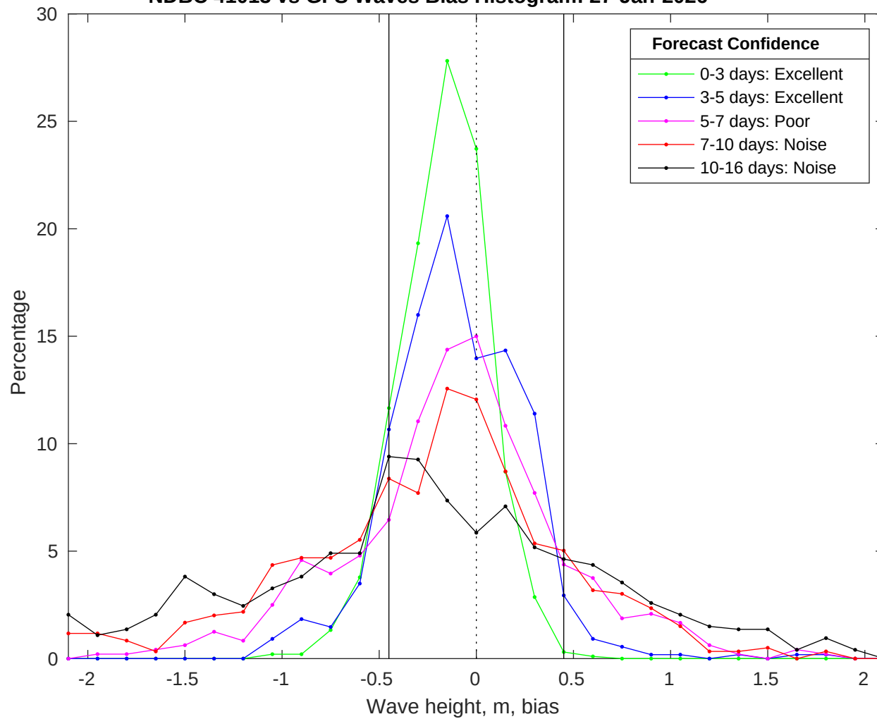
NDBC 41013 vs GFS Waves Bias Histogram: 27-Jan-2026
