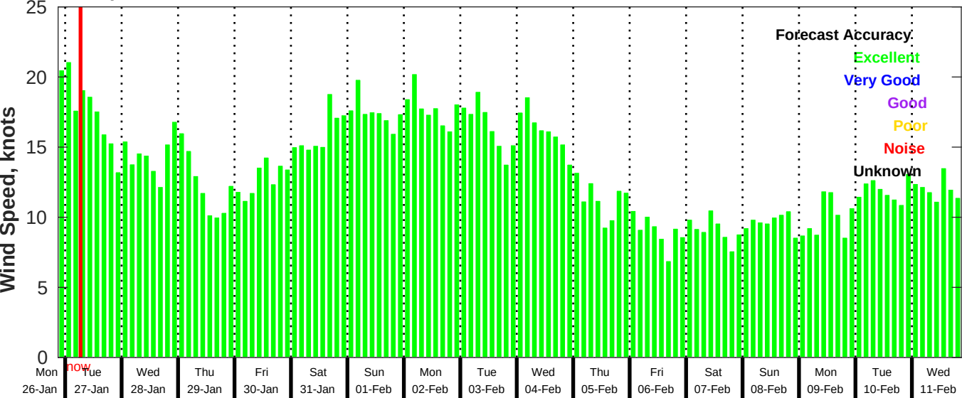
GFS Wind Speed Forecast for NDBC 41040 from 26-Jan-2026 21:00:00 to 11-Feb-2026 21:00:00
