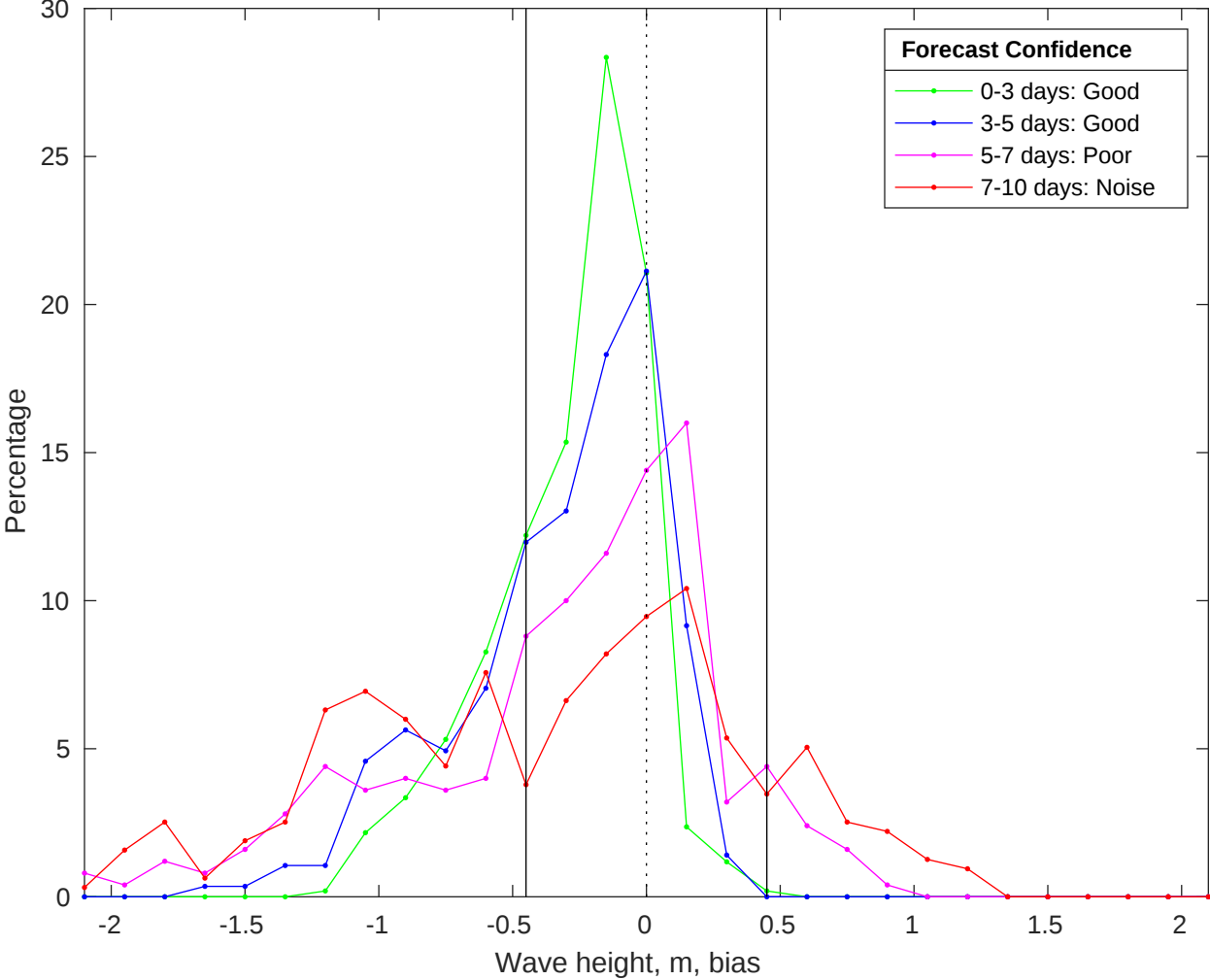
NDBC 42019 vs CMEMS Waves Bias Histogram: 27-Jan-2026
