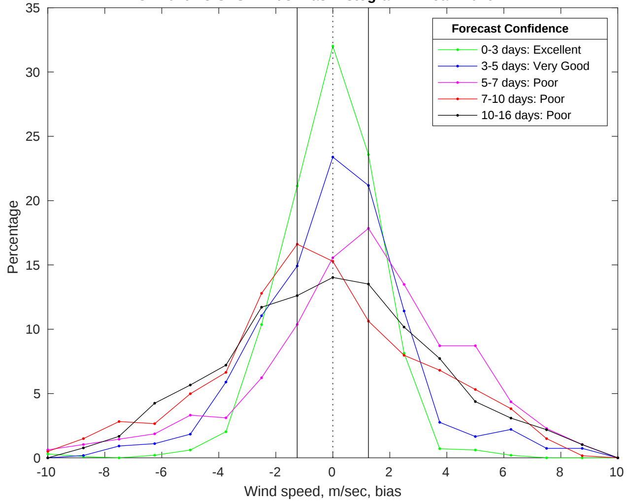
NDBC 42019 vs GFS Winds Bias Histogram: 27-Jan-2026
