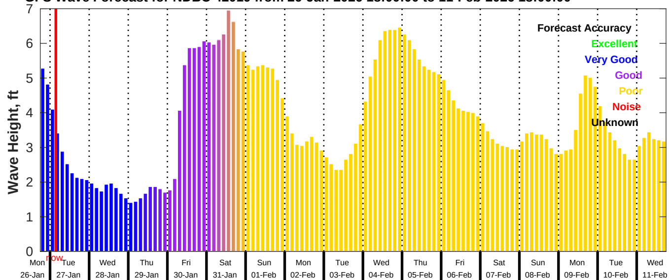
GFS Wave Forecast for NDBC 42019 from 26-Jan-2026 18:00:00 to 11-Feb-2026 18:00:00
