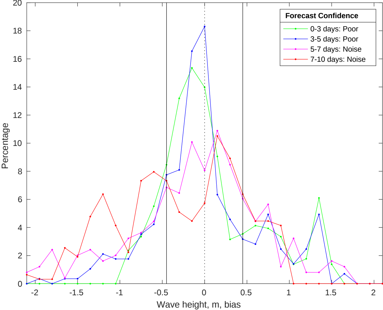
NDBC 42020 vs CMEMS Waves Bias Histogram: 27-Jan-2026
