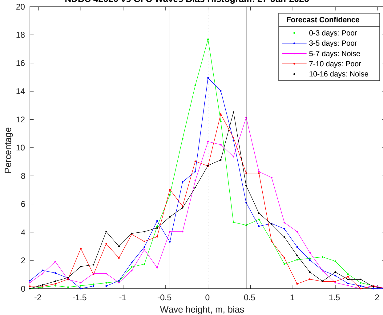
NDBC 42020 vs GFS Waves Bias Histogram: 27-Jan-2026
