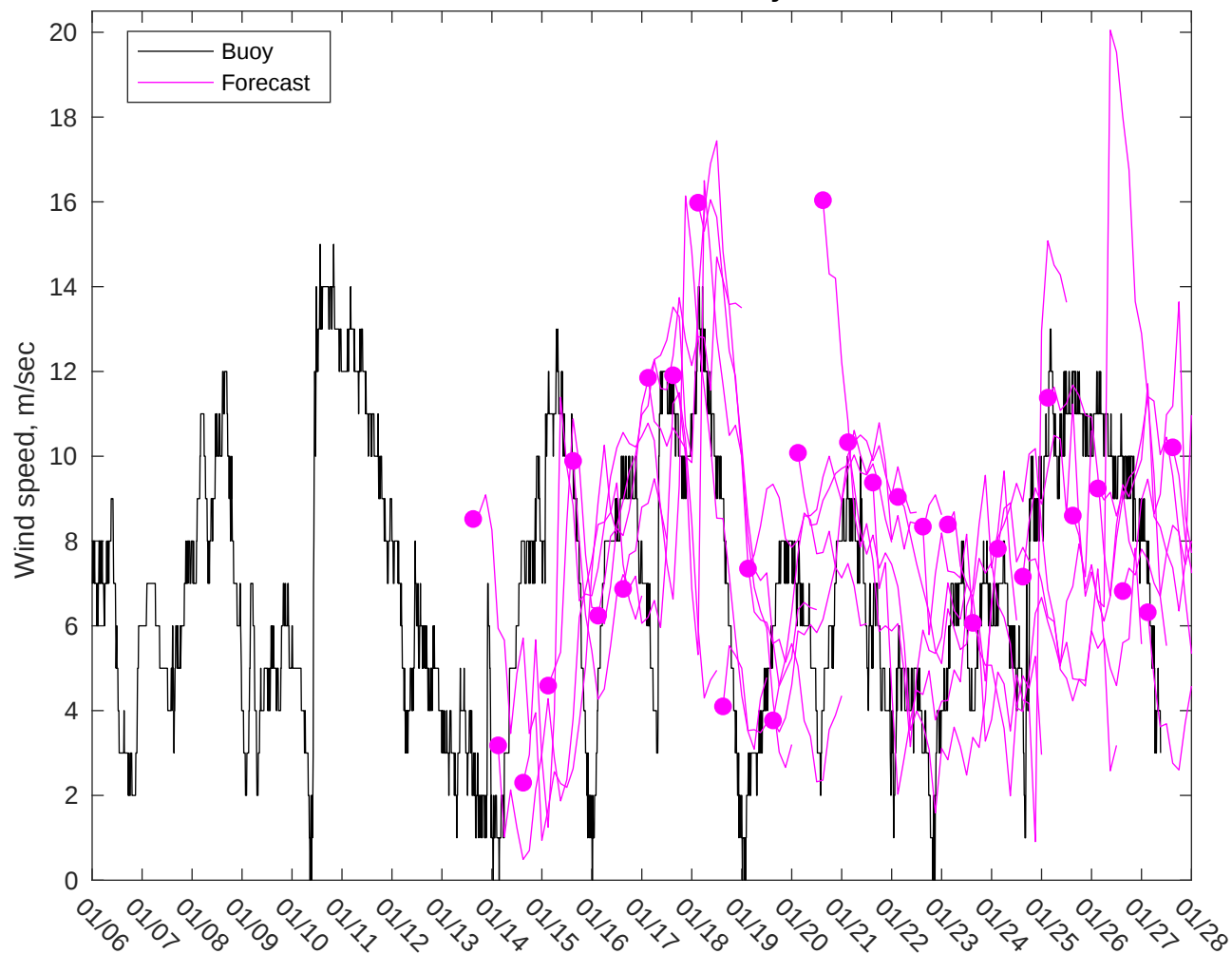
NDBC 42020 vs GFS Winds: 7 to 10 day forecast
