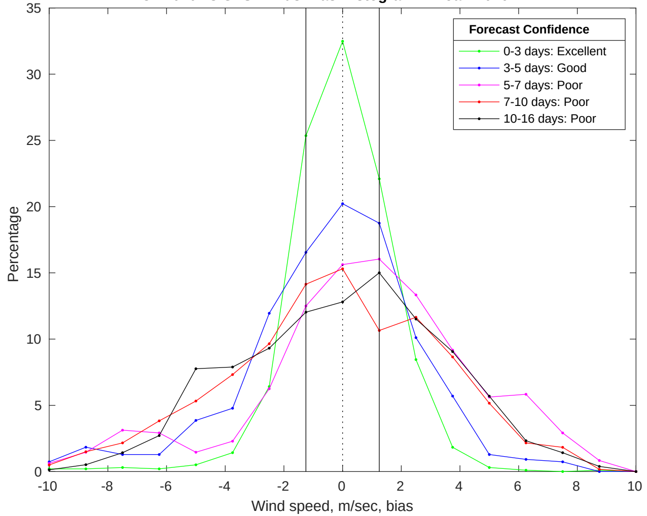
NDBC 42020 vs GFS Winds Bias Histogram: 27-Jan-2026
