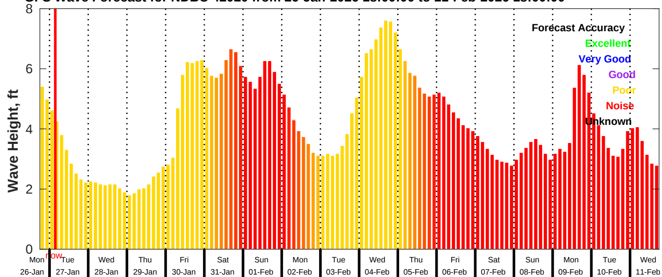
GFS Wave Forecast for NDBC 42020 from 26-Jan-2026 18:00:00 to 11-Feb-2026 18:00:00
